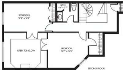
Three Bedroom - Second Floor
